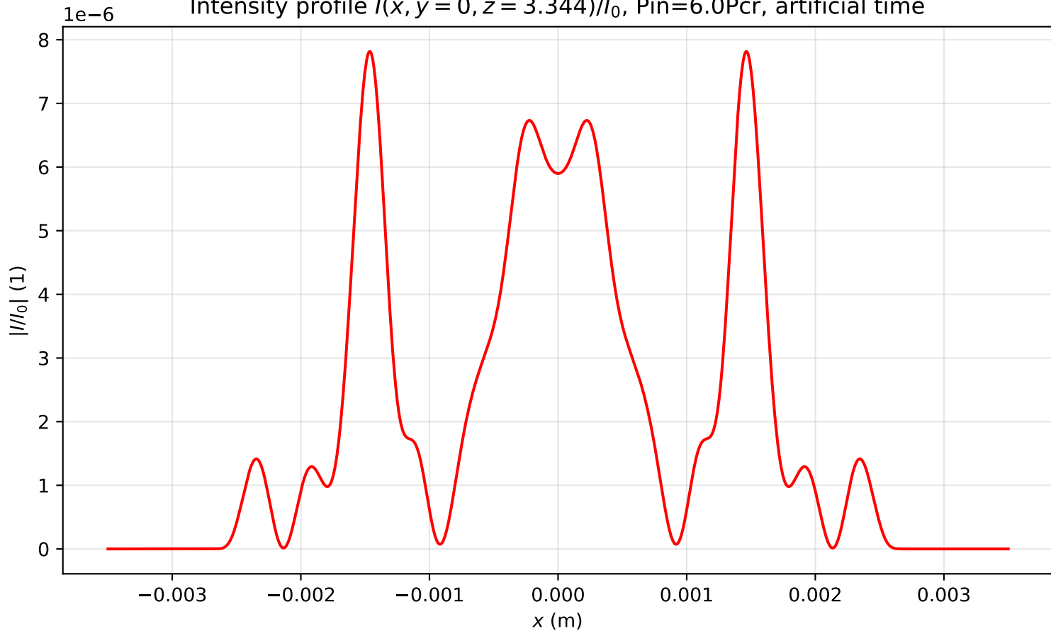
Intensity profile I(x, y = 0, z = 3.344)/I_0 , P_{in}=6.0P_{cr} , artificial time
